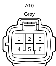
90980-11194 (LED Headlight Type)
