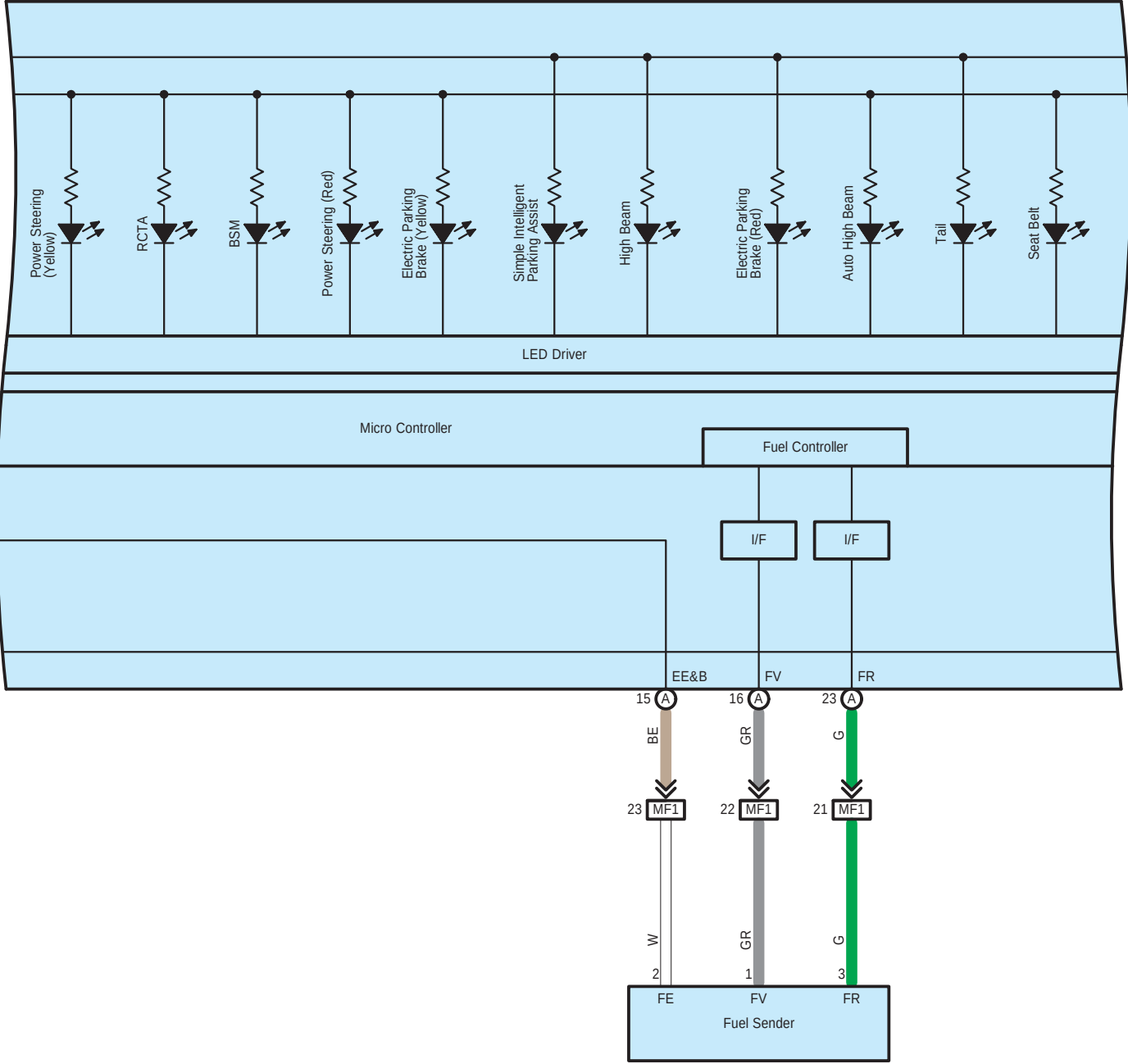
F4(A), F5(B) Combination Meter Assembly
