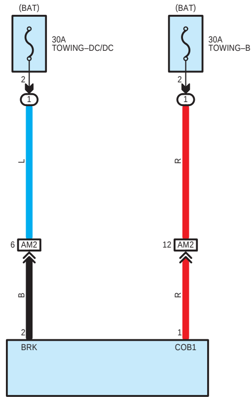
M78 Option Connector (Trailer Towing)
