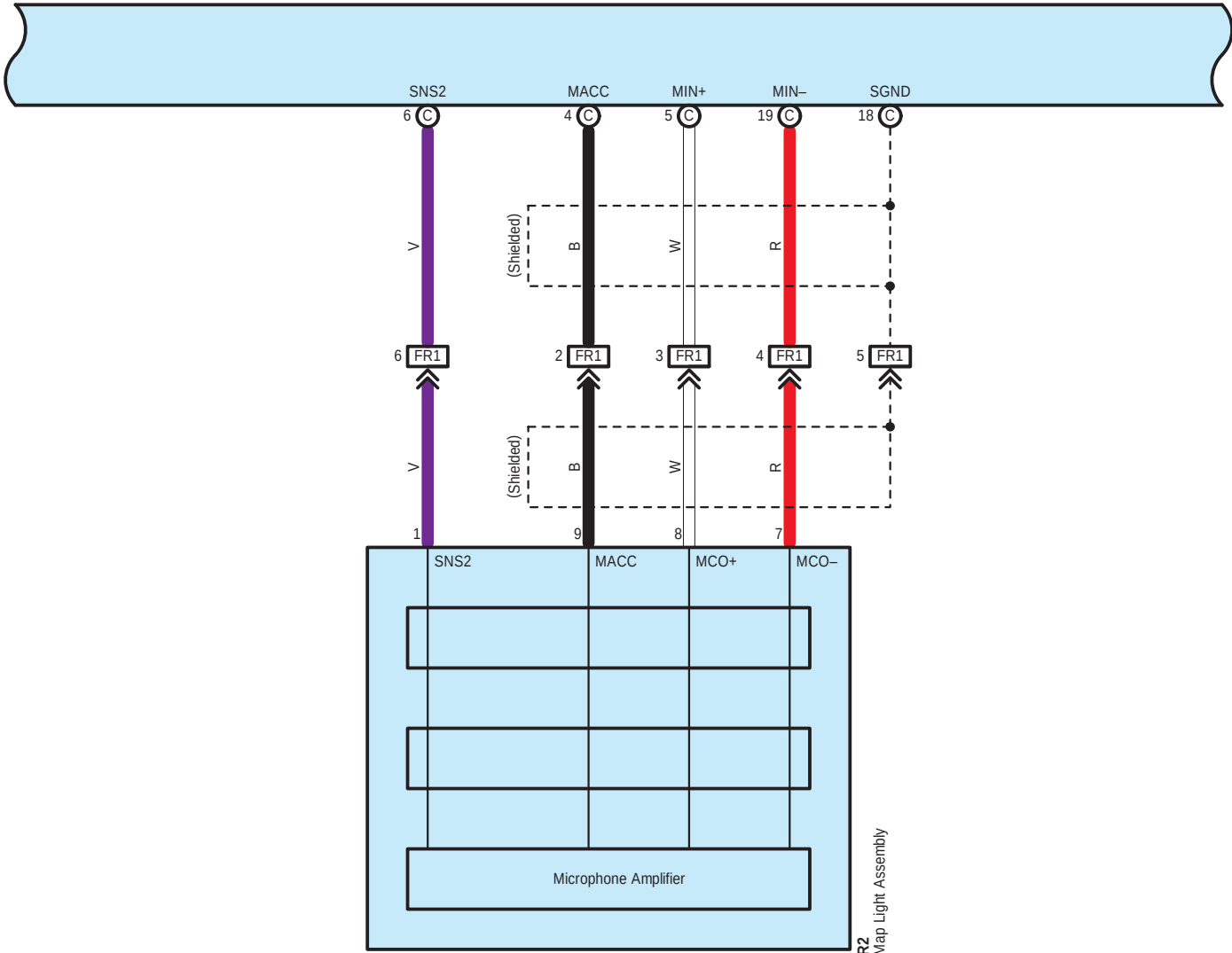
F50(A), F80(B), F125(C), F126(D), F127(E), j2(F), k1(G) Radio & Display Receiver Assembly
