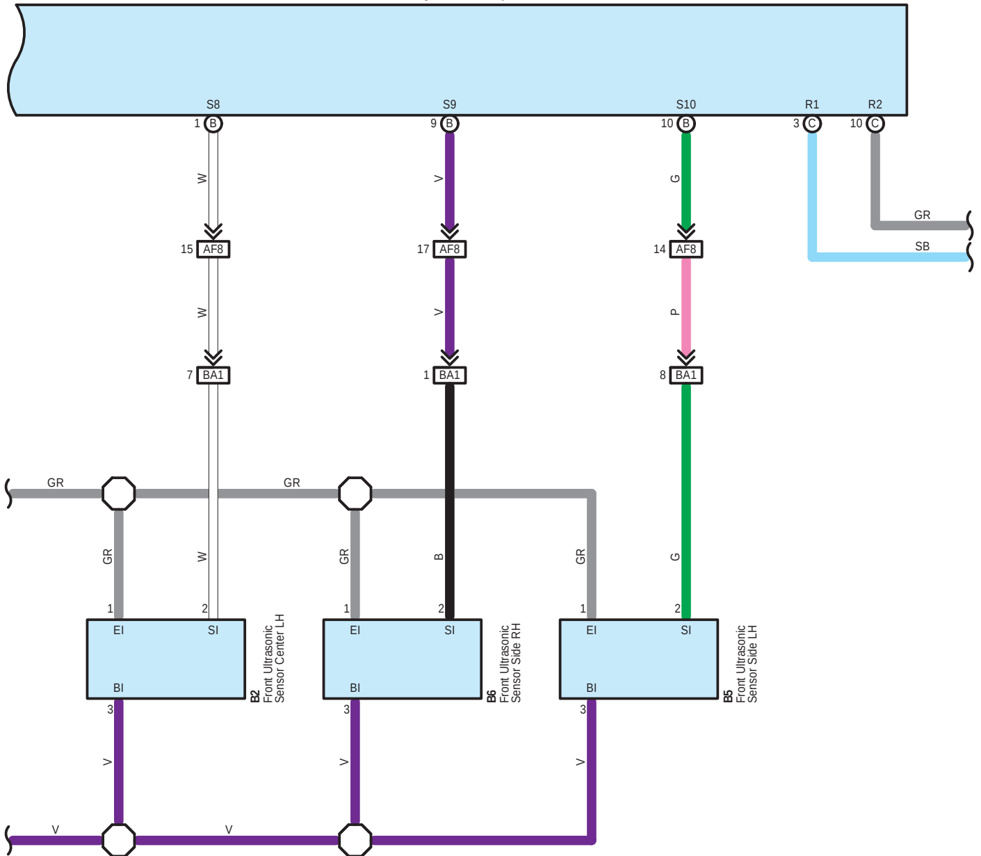
F34(A), F37(B), F38(C) Clearance Warning ECU Assembly
