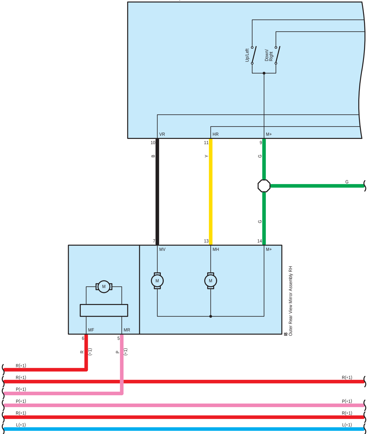
I12 Outer Mirror Switch Assembly
