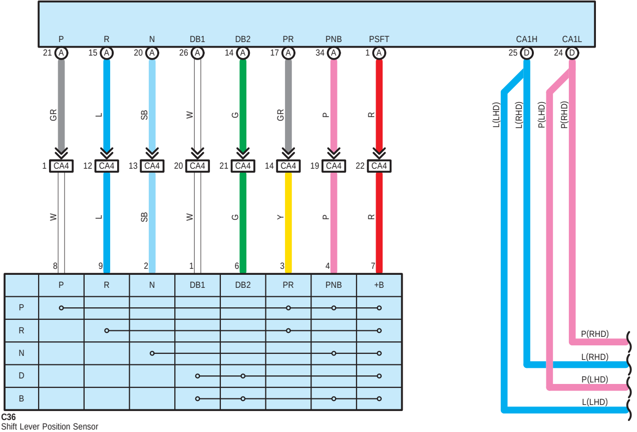
A48(A), F3(D) Hybrid Vehicle Control ECU
