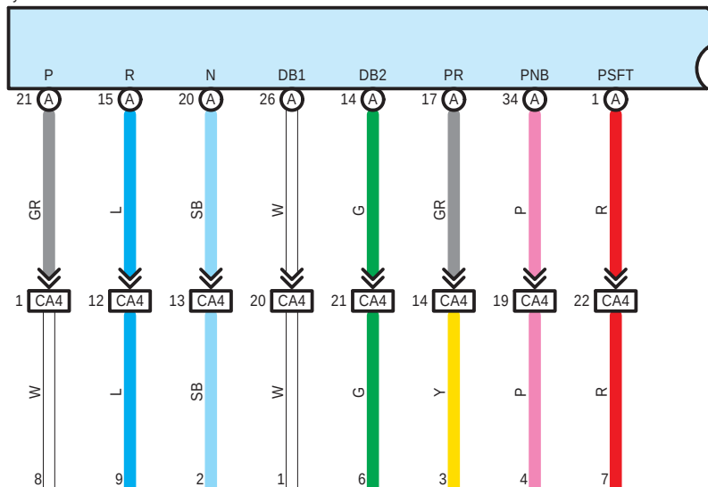
A48(A), F3(D) Hybrid Vehicle Control ECU
