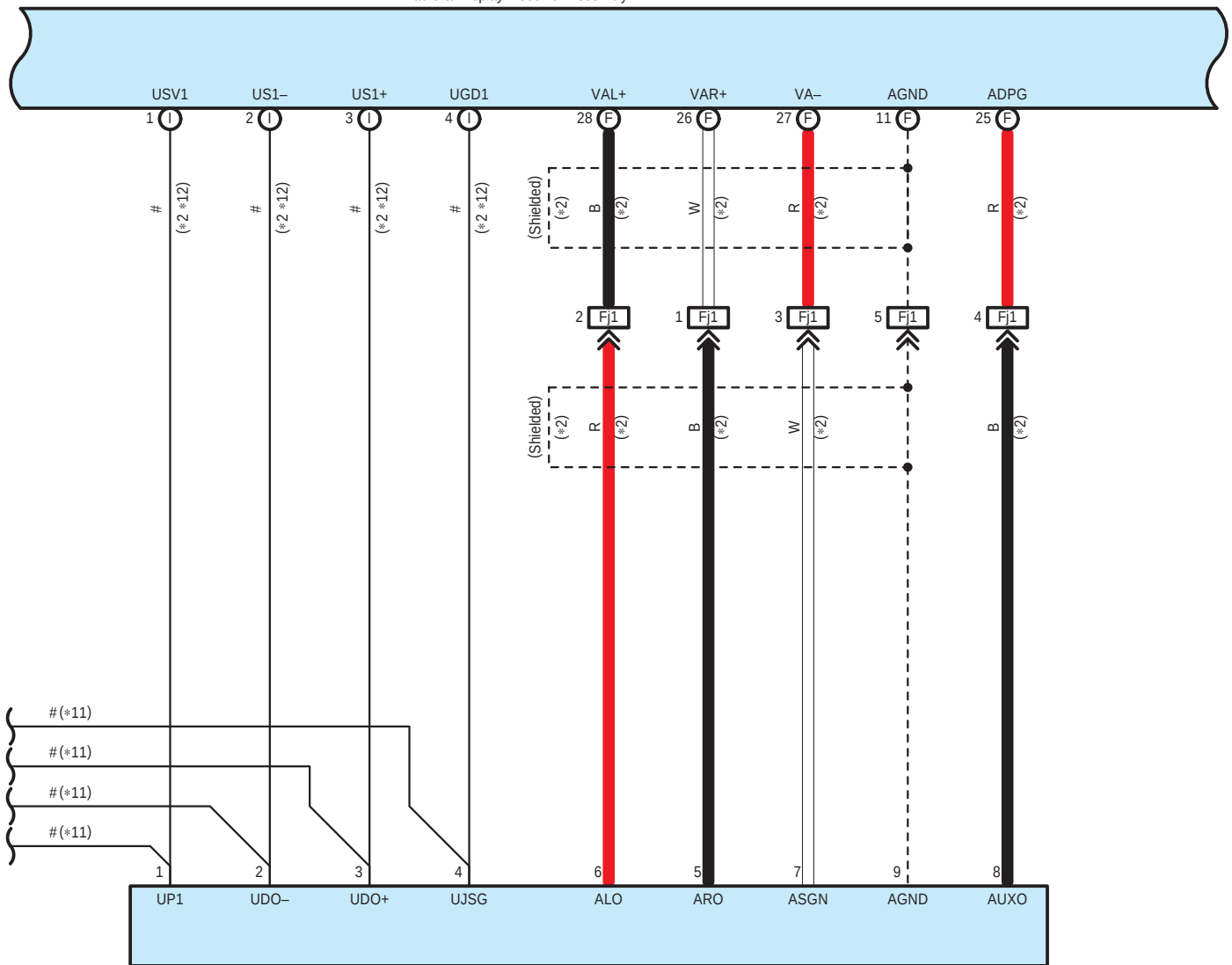
j1 No. 1 Stereo Jack Adapter Assembly
