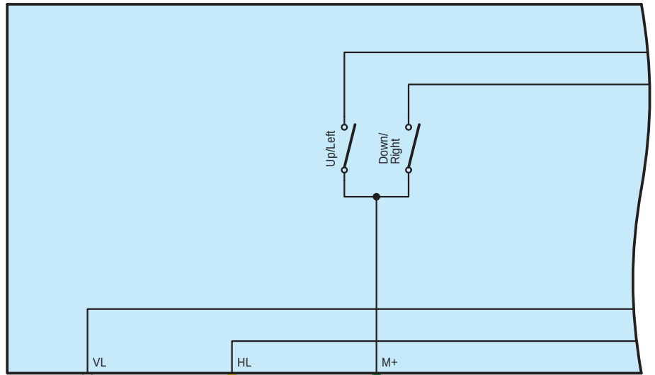
J10 Outer Mirror Switch Assembly
